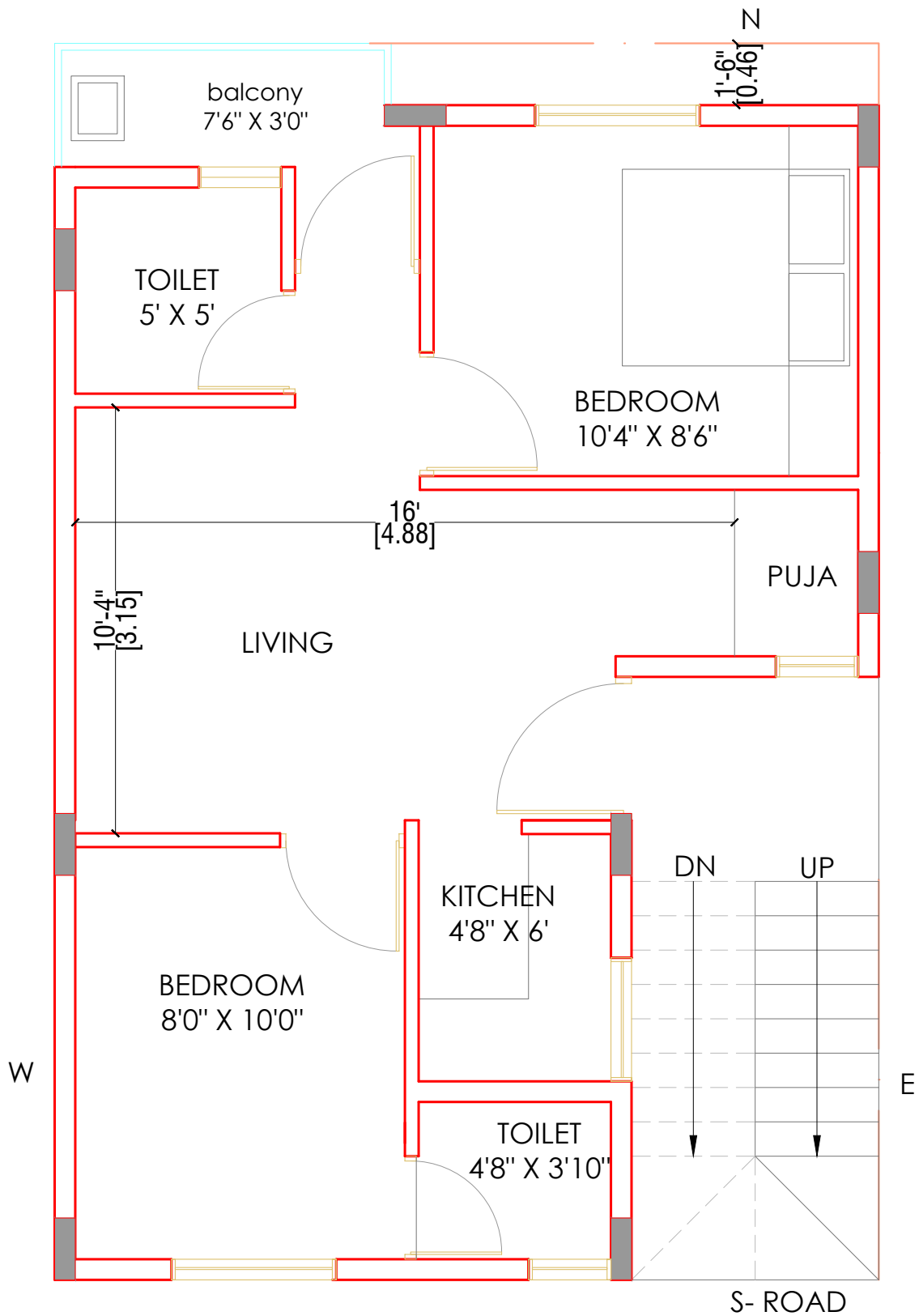
FIRST & SECOND FLOOR PLAN:- 544 SFT BALCONY & UTILITIES:- 36 SFT
